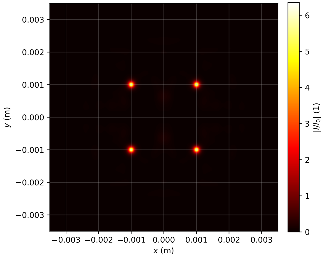
Intensity profile I(x, y, z = 3.582)/I_0 , P_{in}=9.0P_{cr} , artificial time
